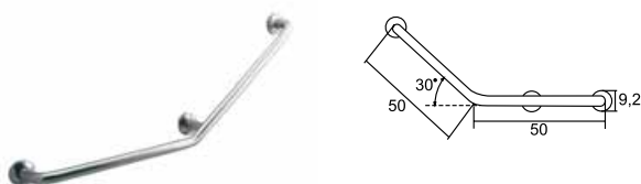
50x50 cm 30° grab rail Barre murale coudeé 50x50 cm. 30°
