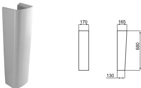
1 ACRO. Pedestal for basin 60 cm. and cloakroom basin 50 cm. . Colonne pour lavabo 60 cm. et lave-mains 50 cm. .
