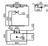
1 80x45 cm wall hung basin with central bowl and overflow. Includes 100041225 - N421040000 fixing kit. With holes for installing towel bar 100123687-N643000039 or 100123688-N643000037 Lavabo 80x45 cm suspendu, avec bac centré et trop-plein
