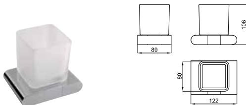
Wall mounted tumbler holder Porte-gobelet fixe
