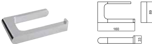
Roll holder without cover Porte-papier sans couvercle
